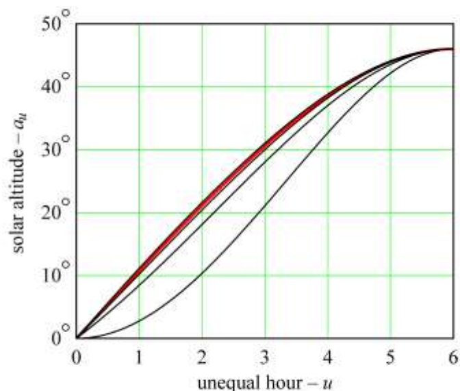
Fig. 9. Five examples where the noon altitude is 46^\circ . The red curve shows the quadrant's understanding of the solar altitude for unequal hours from 0 to 6. At latitude 44^\circ , on the day of an equinox, this exactly matches the actual solar altitude over this period. The lowest curve shows the solar altitude at latitude 67^\circ on a day when the solar declination is 23^\circ . The sun is on the horizon at midnight but otherwise above the horizon for all 24 hours of the day. The errors are large. The other curves are for latitudes 21^\circ , 52^\circ and 62^\circ . The errors are small.
