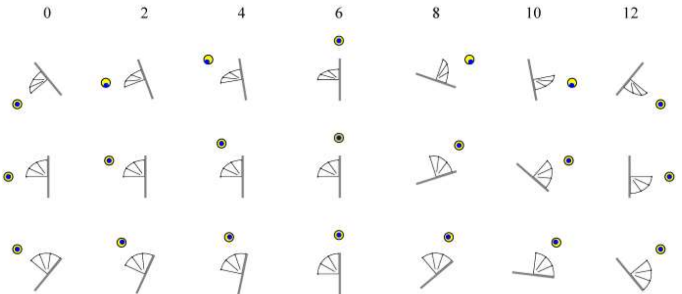
Fig. 5. Each of the three rows of figures shows plan views of the instrument (with south at the top) when making observations at the unequal hours 0, 2, ... 12. In each case, a schematic sun is shown which aligns with the relevant hour line; a blue dot indicates the actual azimuth of the sun at the unequal hour in question. In all cases the local latitude is 52^\circ north. The solar declinations in the three rows are +23^\circ , 0^\circ and -23^\circ so the noon altitudes (and quadrant slopes) are 61^\circ , 38^\circ and 15^\circ .
