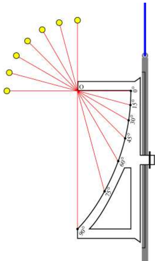
Fig. 2. The gnomon assembly seen in profile.
